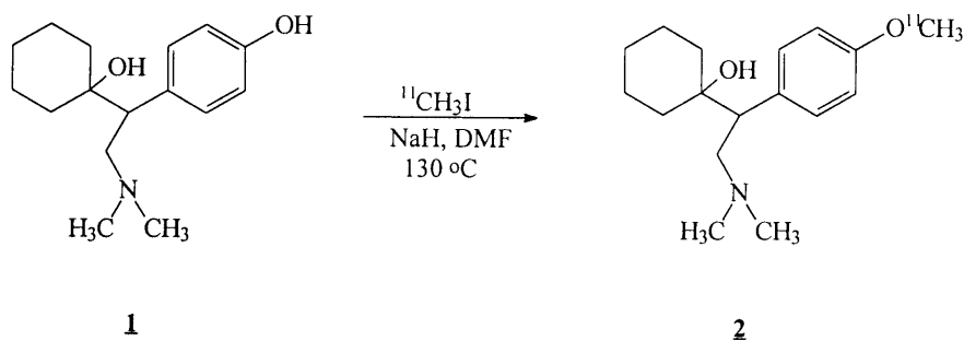
Scheme 1. The synthesis of [ O -methyl- ^{11}\text{C} ]venlafaxine
